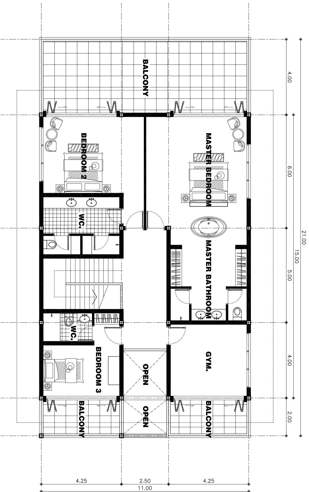
MAIN BUILDING SECOND FLOOR PLAN SCALE 1:100
