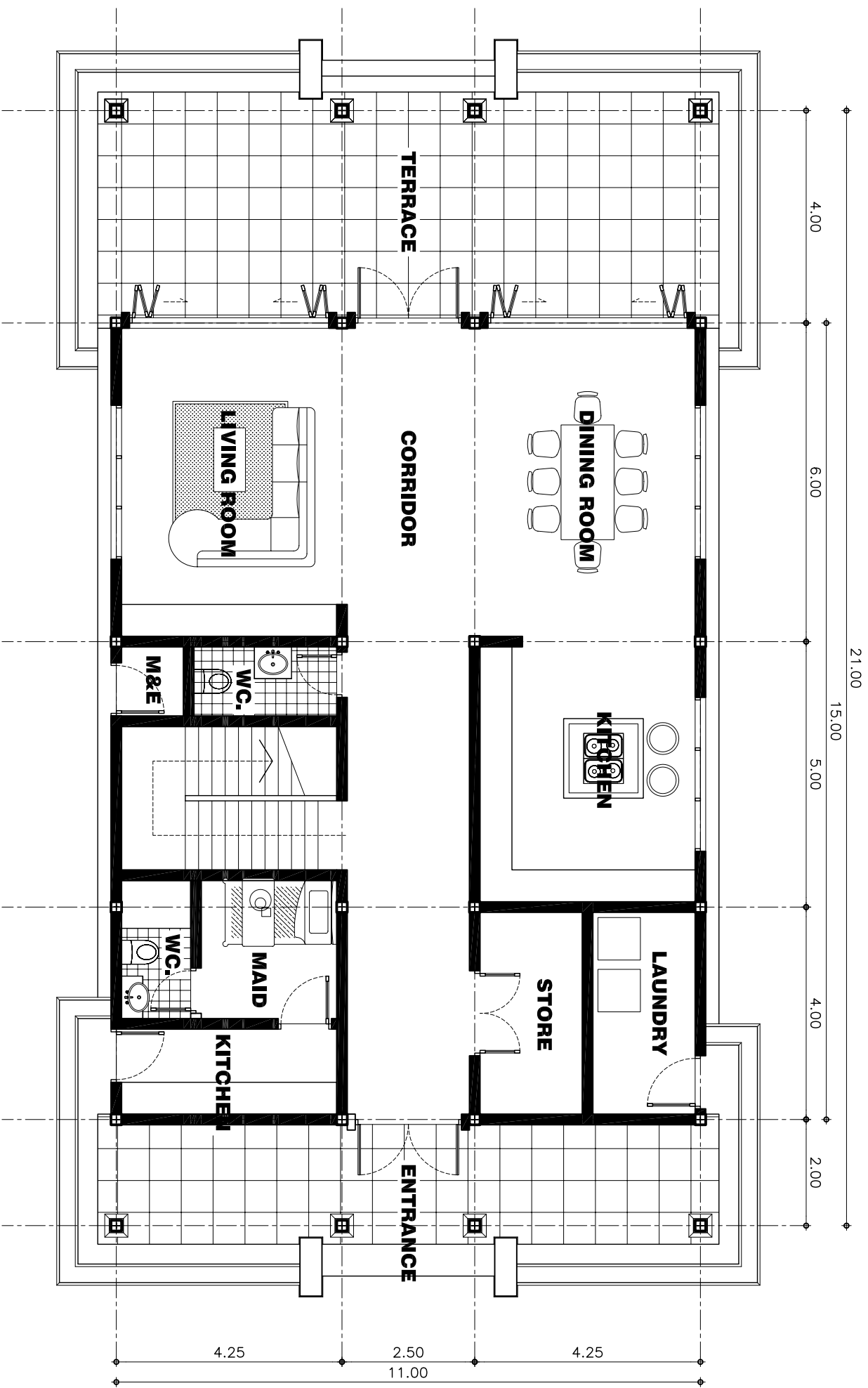
MAIN BUILDING GROUND FLOOR PLAN SCALE 1:100
